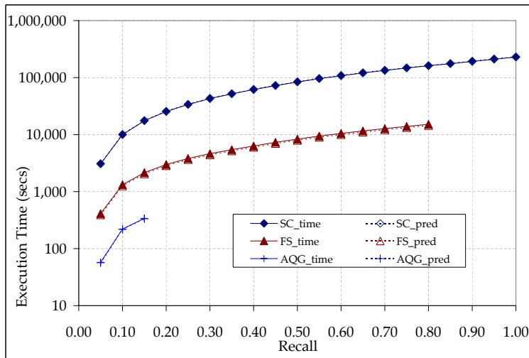
Figure 21: Actual vs. estimated execution times for Task 3 , as a function of the target recall \tau
