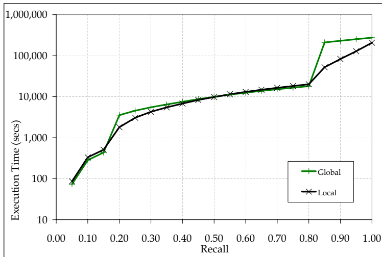
Figure 29: Actual execution times for the global and local optimization approaches, for Task 3 and as a function of the target recall \tau
