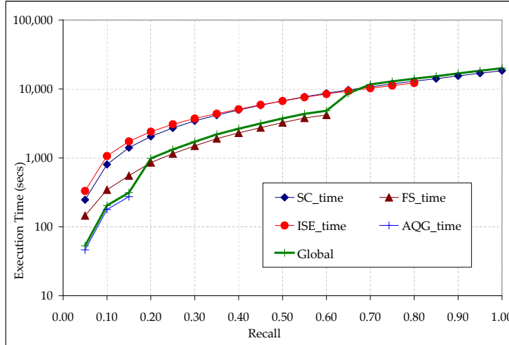
Figure 22: Actual execution times for the four basic execution strategies, as well as for the global optimization approach, for Task 1a and as a function of the target recall \tau
