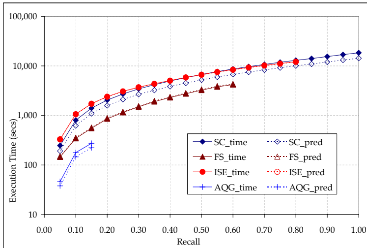
Figure 18: Actual vs. estimated execution times for Task 1a , as a function of the target recall \tau
