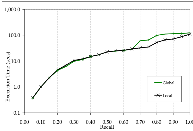
Figure 28: Actual execution times for the global and local optimization approaches, for Task 2 and as a function of the target recall \tau
