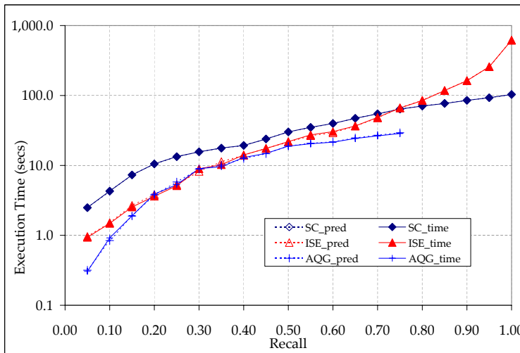
Figure 20: Actual vs. estimated execution times for Task 2 , as a function of the target recall \tau
