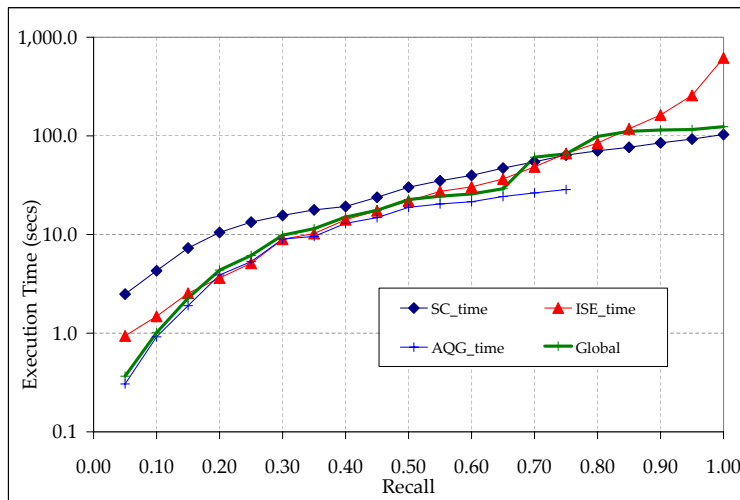
Figure 24: Actual execution times for the three basic execution strategies, as well as for the global optimization approach, for Task 2 and as a function of the target recall \tau
