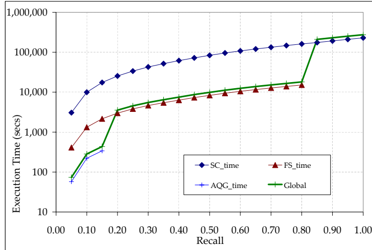
Figure 25: Actual execution times for the three basic execution strategies, as well as for the global optimization approach, for Task 3 and as a function of the target recall \tau
