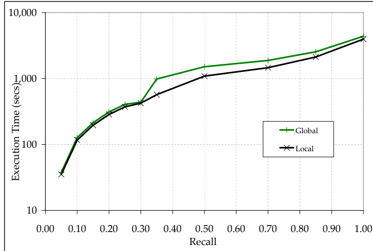
Figure 27: Actual execution times for the global and local optimization approaches, for Task 1b and as a function of the target recall \tau
