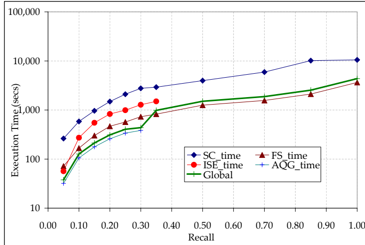
Figure 23: Actual execution times for the four basic execution strategies, as well as for the global optimization approach, for Task 1b and as a function of the target recall \tau
