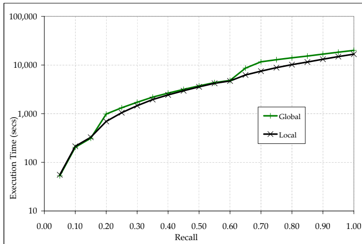
Figure 26: Actual execution times for the global and local optimization approaches, for Task 1a and as a function of the target recall \tau
