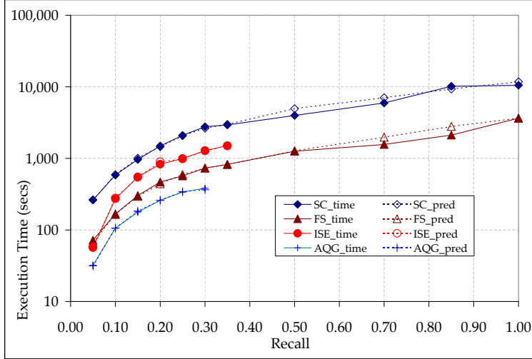
Figure 19: Actual vs. estimated execution times for Task 1b , as a function of the target recall \tau
