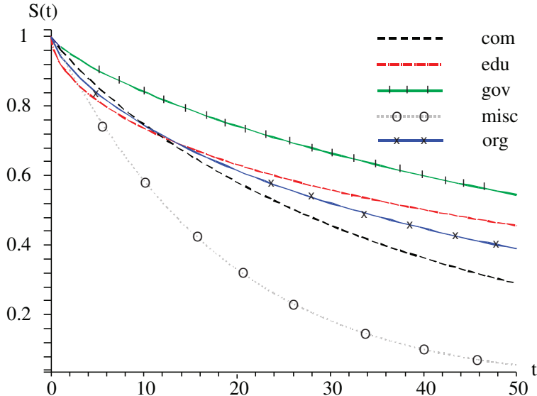
Figure 4: The survival function S(t) for different domains ( |D| = 1000 , \tau = 0.5 , \kappa_1 = 0.1 , QBS summaries).
