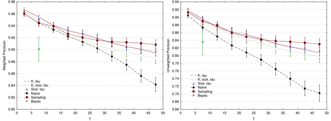
Figure 8: The weighted and unweighted precision of “old” complete content summaries with respect to the “current” ones, as a function of the time T between updates and averaged over each database D in the data set, for different scheduling policies ( \tau = 0.5 ).
