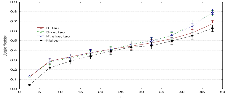
Figure 12: The precision of the updates performed by the different scheduling algorithms, as a function of the average time between updates T and for \tau = 0.5 , where the \kappa_1 feature is computed using QBS summaries.
