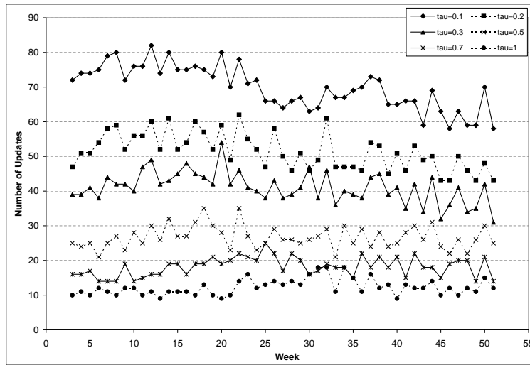
Figure 19: The number of updates performed by the Bayes policy in different weeks, for different values of the change sensitivity threshold \tau and for FPS summaries.
