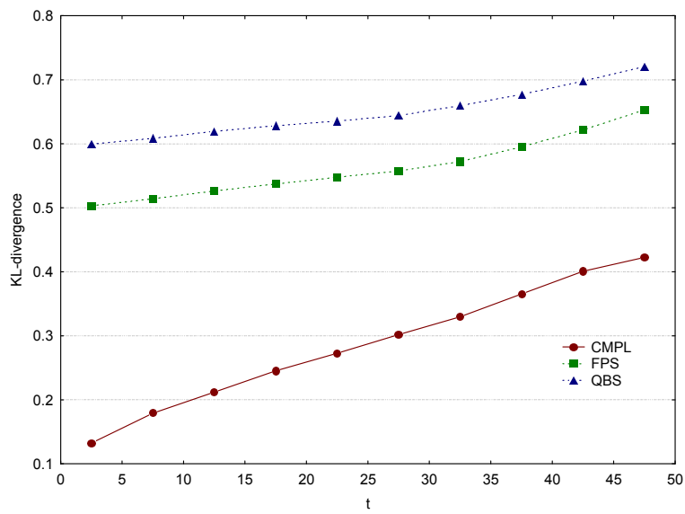
Figure 3: The KL divergence of the content summary O(D, t) ( CMPL ), and of the approximate content summaries \hat{O}(D, t) ( QBS and FPS ), with respect to the “current” content summary C(D) , as a function of time t and averaged over each database D in the data set.
