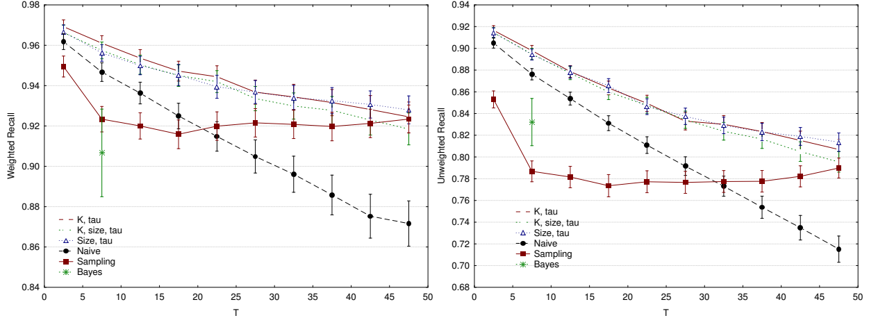
Figure 6: The weighted and unweighted recall of “old” complete content summaries with respect to the “current” ones, as a function of the time T between updates and averaged over each database D in the data set, for different scheduling policies ( \tau = 0.5 ).
