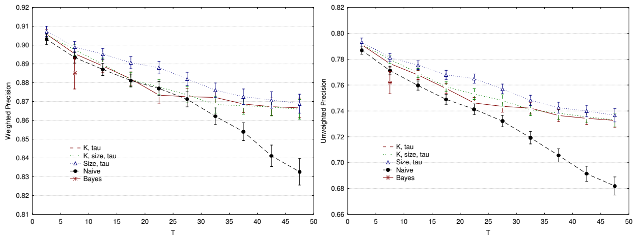
Figure 16: The weighted and unweighted precision of “old” FPS content summaries with respect to the “current” ones, as a function of the time T between updates and averaged over each database D in the data set, for different scheduling policies ( \tau = 0.5 ).
