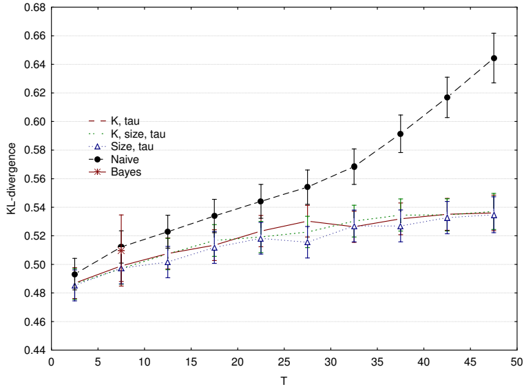
Figure 17: The KL divergence of “old” FPS content summaries with respect to the “current” ones, as a function of the time T between updates and averaged over each database D in the data set, for different scheduling policies ( \tau = 0.5 ).
