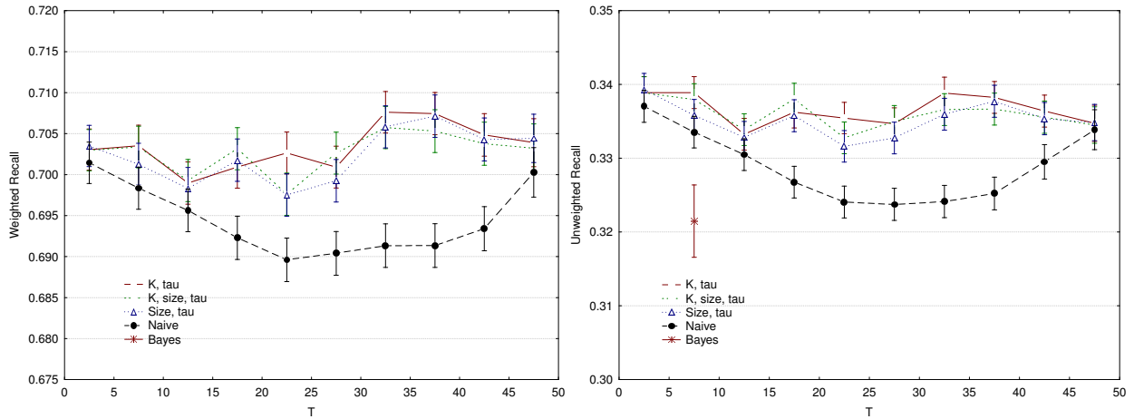
Figure 7: The weighted and unweighted recall of “old” QBS content summaries with respect to the “current” ones, as a function of the time T between updates and averaged over each database D in the data set, for different scheduling policies ( \tau = 0.5 ).
