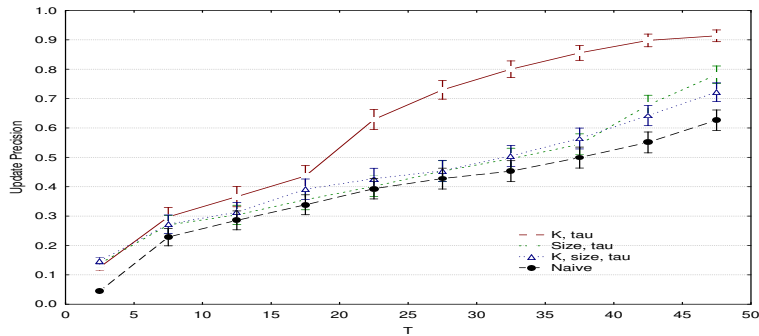
Figure 13: The precision of the updates performed by the different scheduling algorithms, as a function of the average time between updates T and \tau = 0.5 , where the \kappa_1 feature is computed using FPS summaries.
