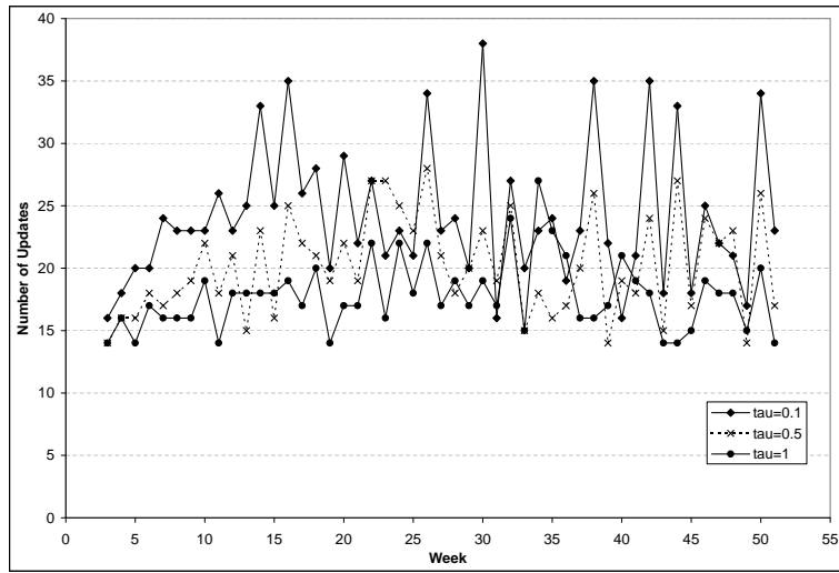
Figure 14: The number of updates performed by the Bayes policy in different weeks, for different values of the change sensitivity threshold \tau and for complete content summaries.
