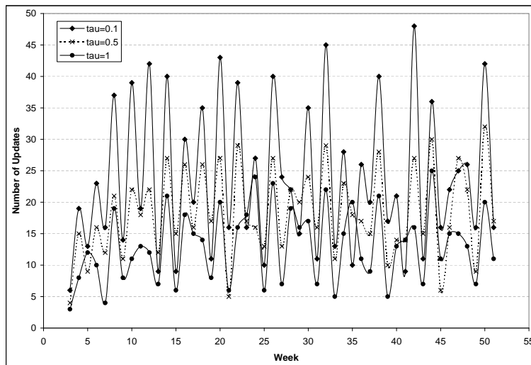
Figure 18: The number of updates performed by the Bayes policy in different weeks, for different values of the change sensitivity threshold \tau and for QBS summaries.
