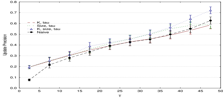
Figure 11: The precision of the updates performed by the different scheduling algorithms, as a function of the average time between updates T and \tau = 0.5 , where the \kappa_1 feature is computed using complete summaries.
