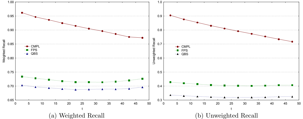
Figure 1: The weighted and unweighted recall of content summary O(D, t) ( CMPL ), and of the approximate content summaries \hat{O}(D, t) ( QBS and FPS ), with respect to the “current” content summary C(D) , as a function of time t and averaged over each database D in the data set.
