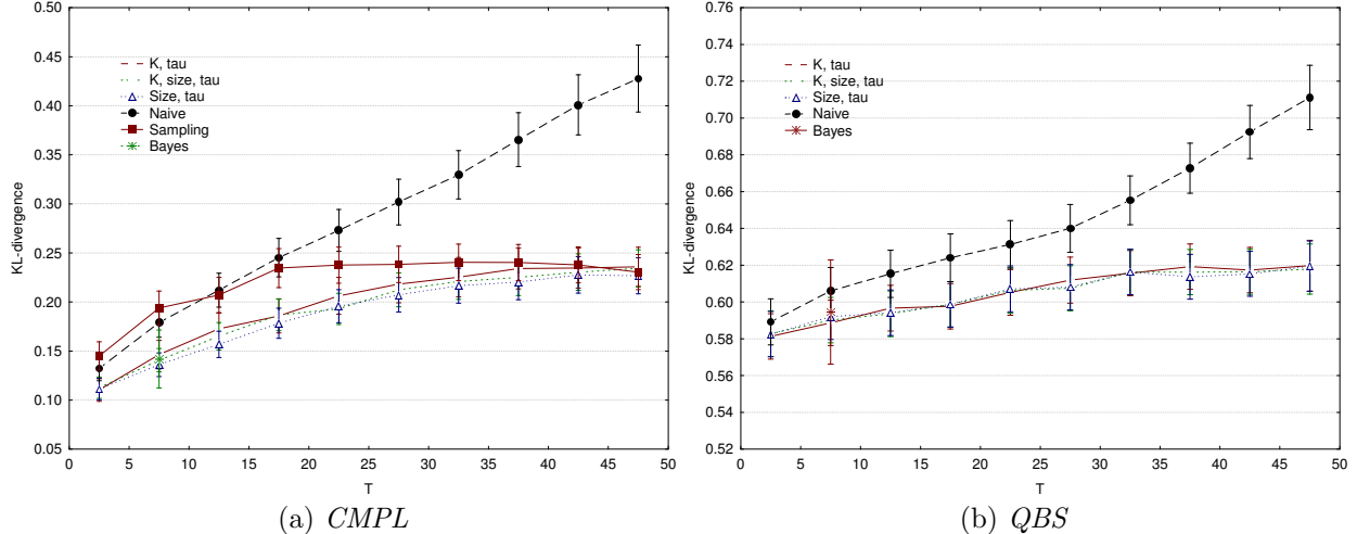
Figure 10: The KL divergence of “old” complete and QBS content summaries with respect to the “current” ones, as a function of the time T between updates and averaged over each database D in the data set, for different scheduling policies ( \tau = 0.5 ).
