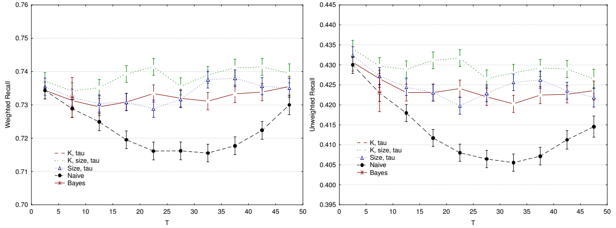
Figure 15: The weighted and unweighted recall of “old” FPS content summaries with respect to the “current” ones, as a function of the time T between updates and averaged over each database D in the data set, for different scheduling policies ( \tau = 0.5 ).
