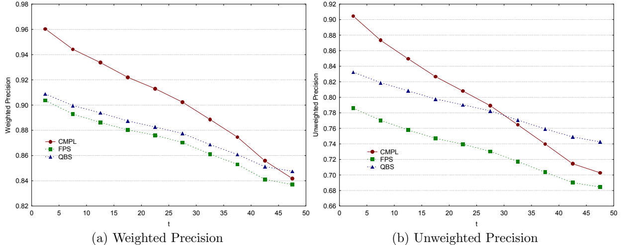
Figure 2: The weighted and unweighted precision of content summary O(D, t) ( CMPL ), and of the approximate content summaries \hat{O}(D, t) ( QBS and FPS ), with respect to the “current” content summary C(D) , as a function of time t and averaged over each database D in the data set.
