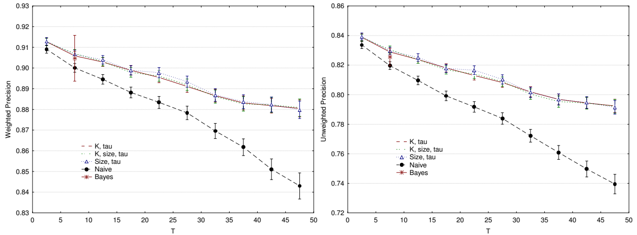
Figure 9: The weighted and unweighted precision of “old” QBS content summaries with respect to the “current” ones, as a function of the time T between updates and averaged over each database D in the data set, for different scheduling policies ( \tau = 0.5 ).
