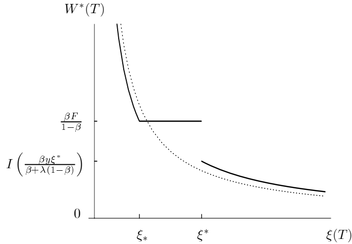
Figure 1: The borrower's time- T optimal wealth, W^*(T) (solid plot), and the time- T B-policy, W^B(T) = I(y^B\xi(T)) (dotted plot), when debt maturity coincides with the borrower's planning horizon ( T = T' ).
