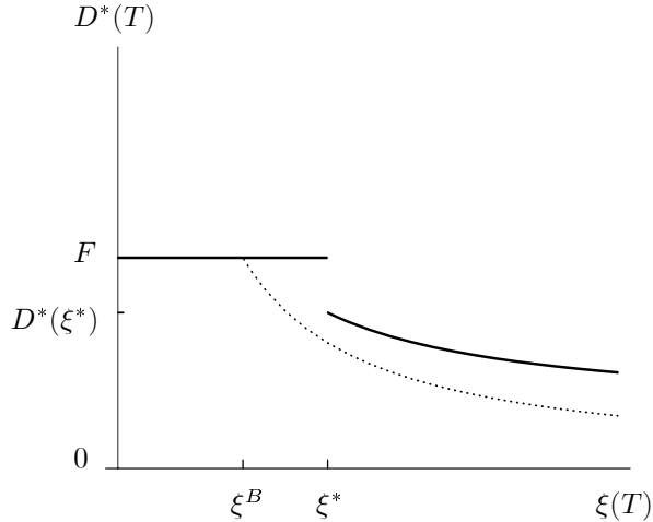
Figure 3: The time- T debt payoff with costly default (solid plot), and with costless default (dotted plot), when debt maturity coincides with the borrower's planning horizon ( T = T' ).
