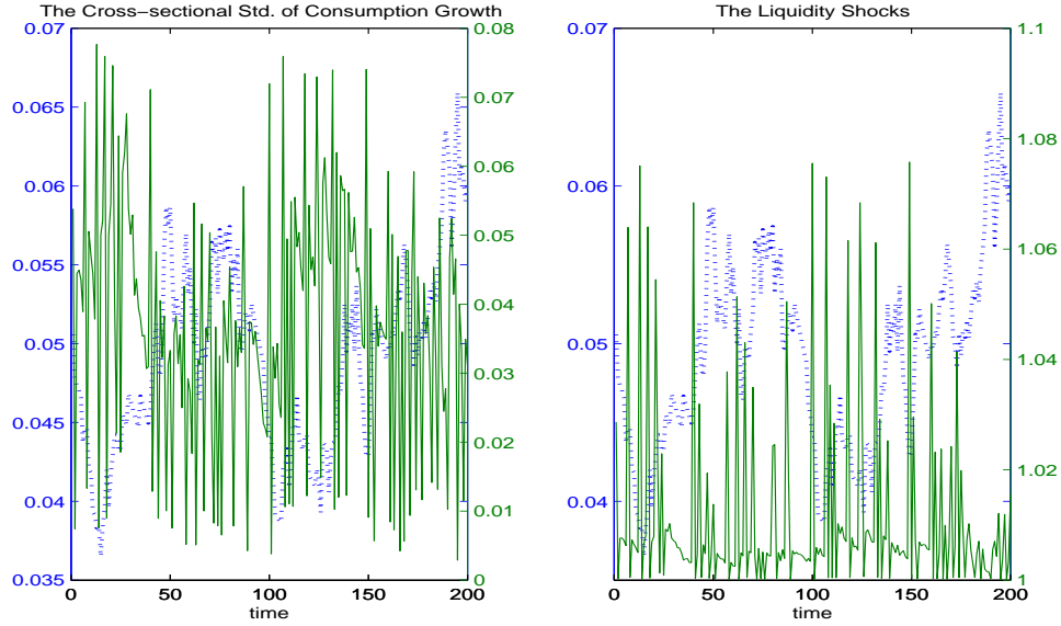
Figure 3: The Standard Deviation of Consumption Growth, Liquidity Shocks and my The dotted line is the collateral ratio: \beta is .95, \gamma is 8 and \varepsilon is .151 ratio: \beta is .95. The left panel plots my against the cross-sectional std. of consumption growth (right axis). The right panel plots my against the aggregate liquidity shock g (right axis).
