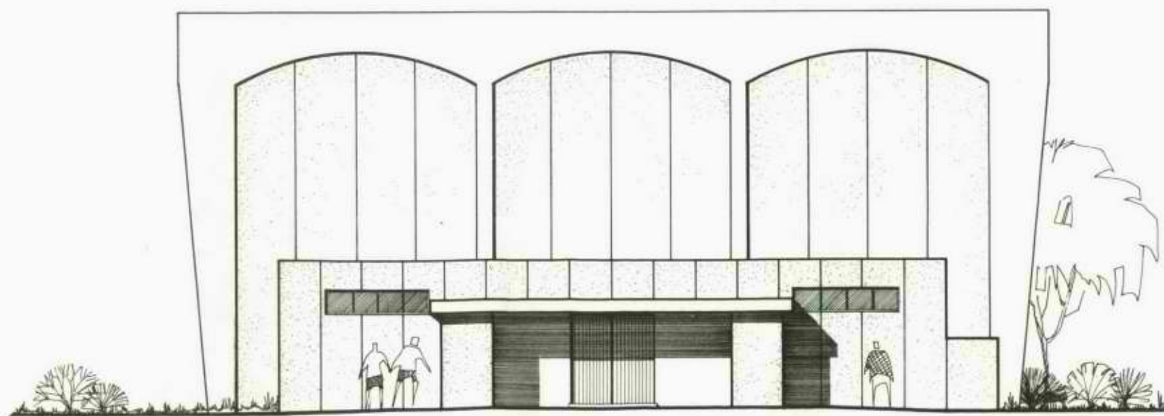
EAST ELEVATION
