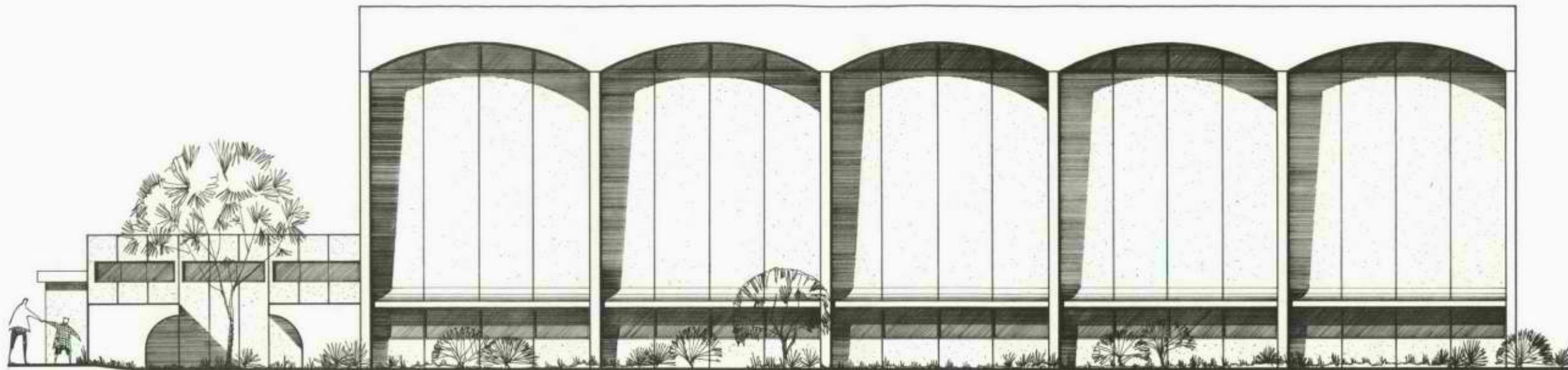
NORTH ELEVATION
