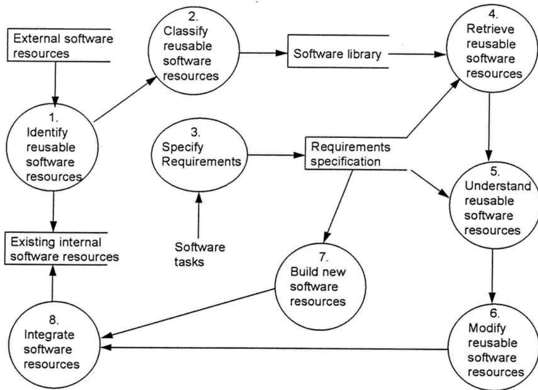
Figure 2. A Model of Reuse-Based System Development
