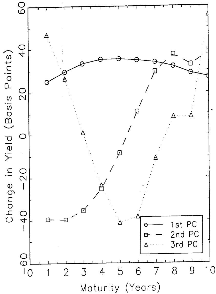
Figure 6: Factor Loadings. Figure 6 presents the factor loadings of three factor model. Three factors are extracted from estimated spot rates with maturities from one to ten years for the period April 27, 1990 to May 17, 1996, by using the principal component method.
