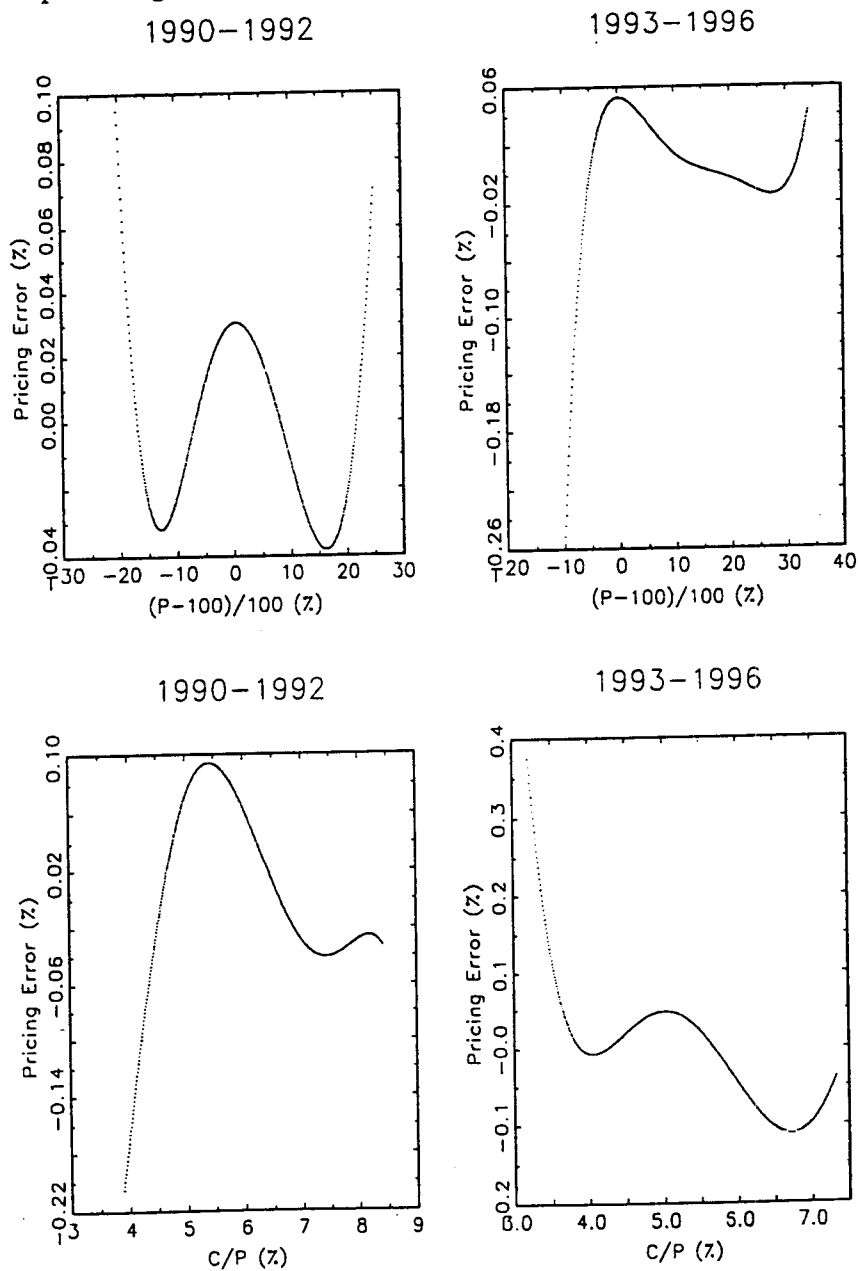
Figure 4: Coupon Effect:Nonlinear regression. Figure 4 presents the empirical estimates of nonlinear regression for the relation between the relative fitted pricing error and coupon variables such as current income and the “par-ness” of a bond. The estimation is performed by Legendre orthogonal polynomials, Current income is measured as a ratio between a coupon and a bond price including accrued interests. The the ‘par-ness’ of a bond is measured by (Price - 100)/100 . Both numbers are in percentage.
