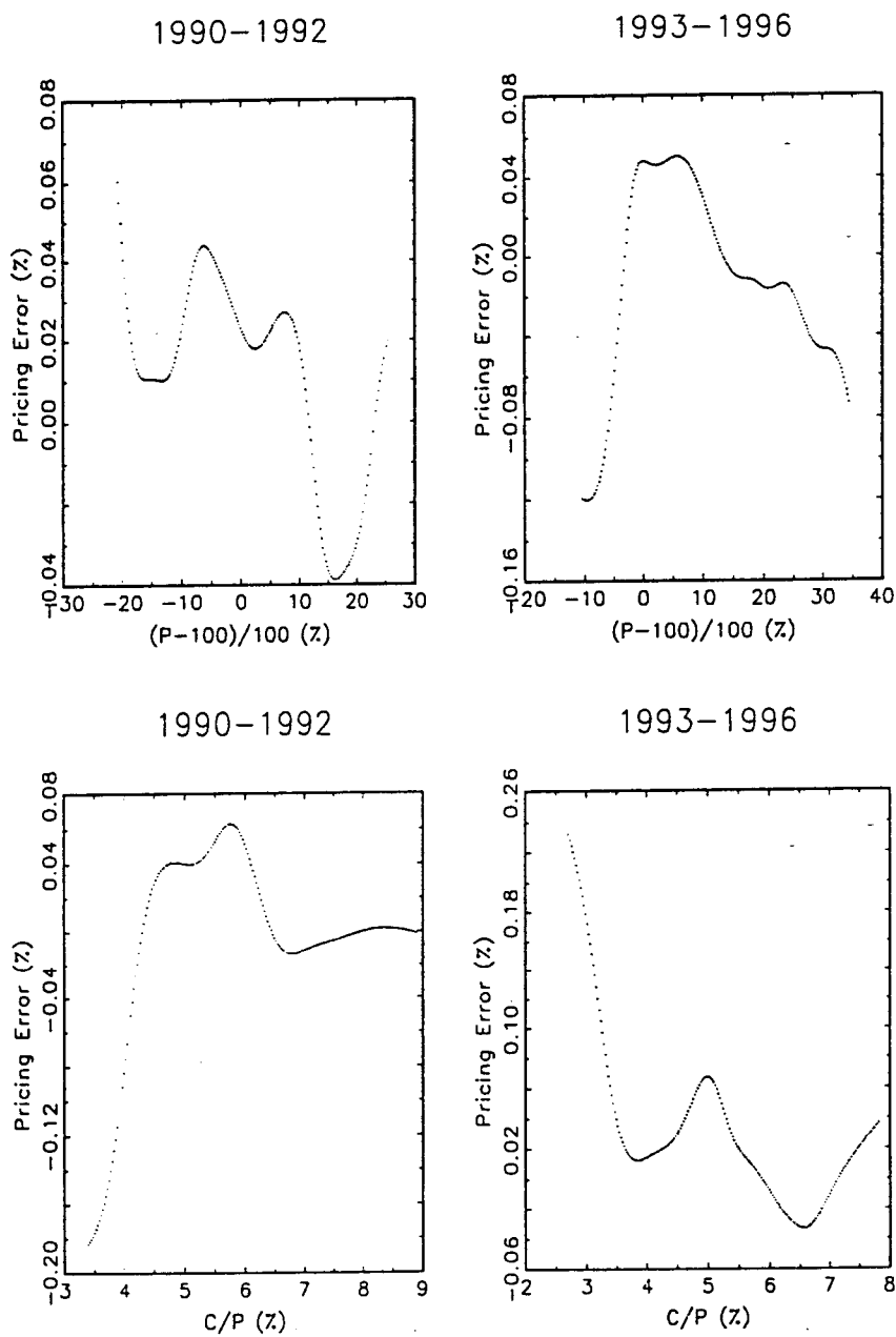
Figure 5: Coupon Effect: Nonparametric Kernel Regression. Figure 5 presents the empirical estimates of nonparametric Kernel regression for the relation between the relative fitted pricing error and coupon variables such as current income and the “par-ness” of a bond. Current income is measured as a ratio between a coupon and a bond price including accrued interests. The “par-ness” of a bond is measured by (Price - 100)/100 . Both numbers are in percentage.
